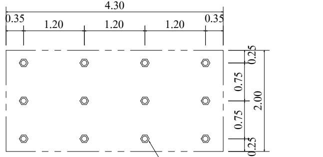
PLAN SHOW LAY-OUT OF PILING SCALE 1 : 100
