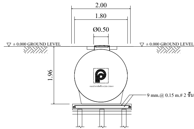
SIDE VIEW SCALE 1 : 100
