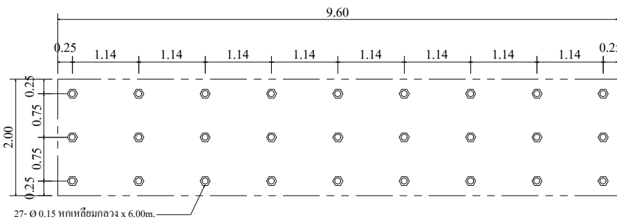
SHOW LAY-OUT OF PILING SCALE 1 : 100
