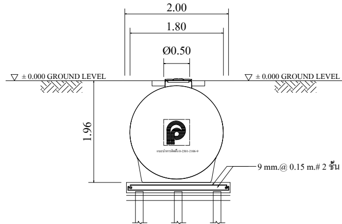
SIDE VIEW SCALE 1 : 100
