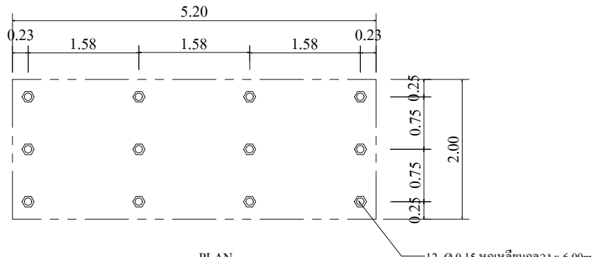
PLAN SHOW LAY-OUT OF PILING SCALE 1 : 100
