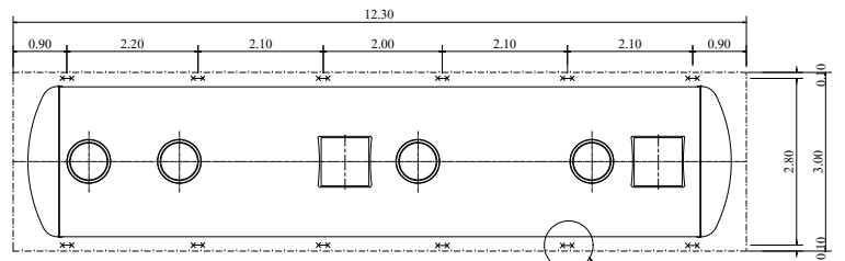
PLAN SCALE 1 : 100 SHOW LAY-OUT OF STEEL ANCHOR STRIP
