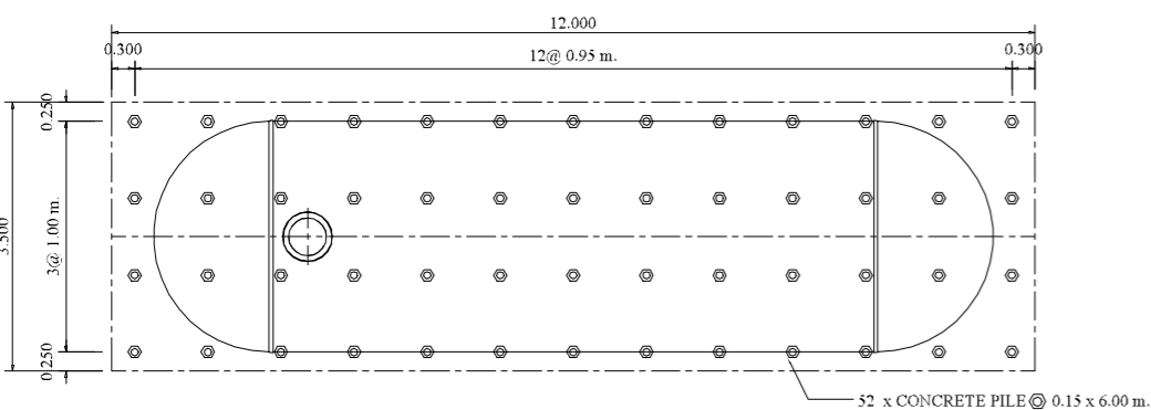
PLAN OF FOUNDATION SCALE : 1:100
