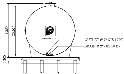
RIGHT VIEW
