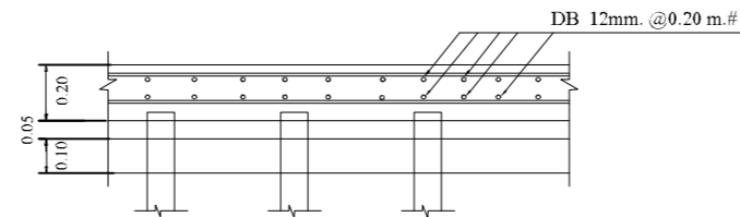
FIG.1 FOUNDATION DETAIL. NOT TO SCALE
