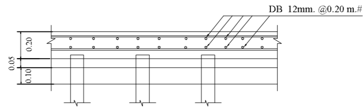
FIG.1 FOUNDATION DETAIL. NOT TO SCALE
