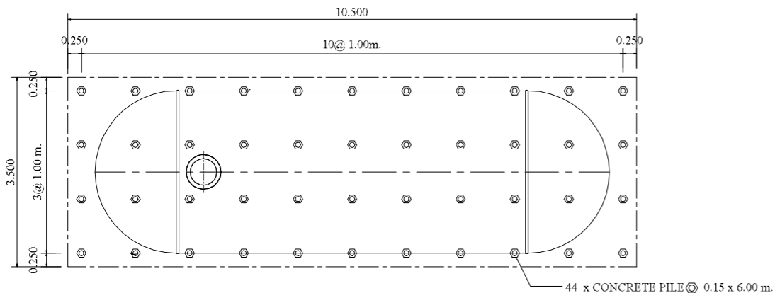
PLAN OF FOUNDATION SCALE : 1:100
