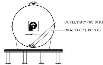
RIGHT VIEW
