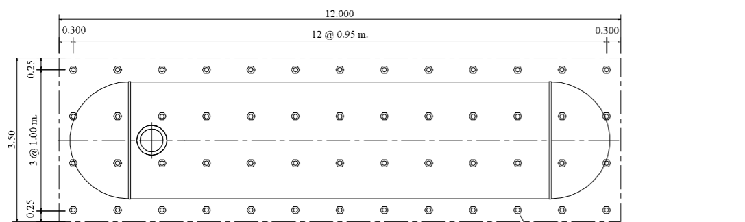
PLAN OF FOUNDATION SCALE : 1:100
