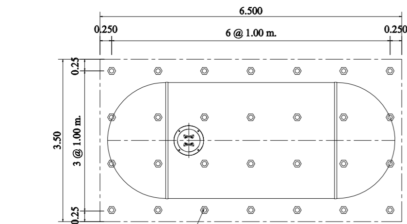
PLAN OF FOUNDATION
