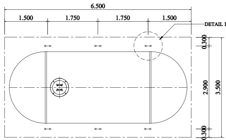
PLAN OF STEEL ANCHOR STRIP
