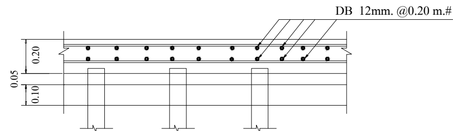
FIG.1 FOUNDATION DETAIL.
