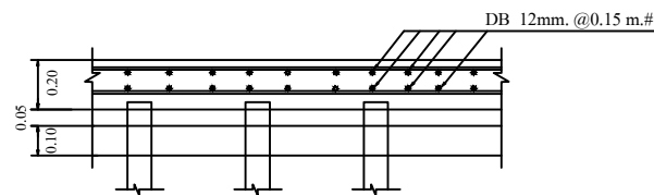
FIG.1 FOUNDATION DETAIL. NOT TO SCALE
