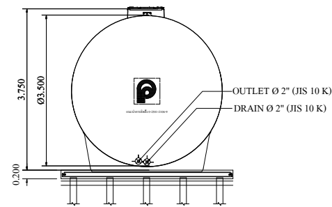
RIGHT VIEW
