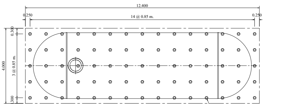
PLAN OF FOUNDATION SCALE : 1:100
