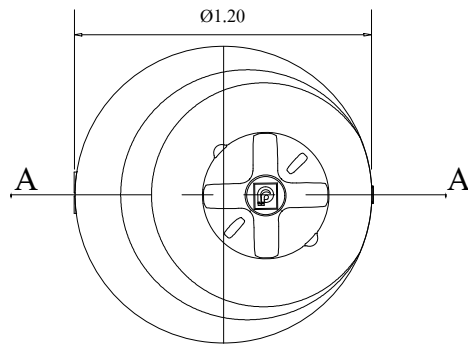
TOP VIEW SCALE 1 : 100
