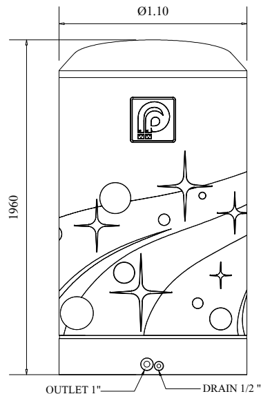
FRONT VIEW SCALE 1 : 100
