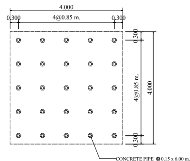
PLAN OF FOUNDATION SCALE : 1:100
