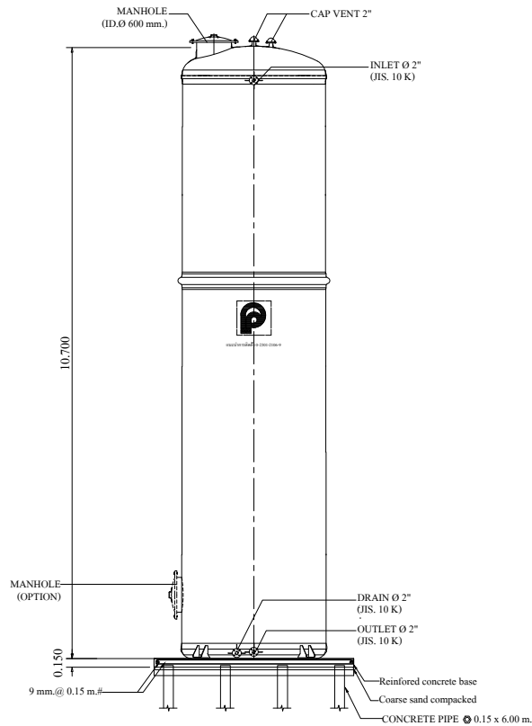
FRONT VIEW SCALE : 1:100
