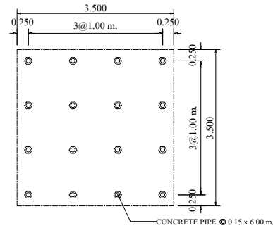
PLAN OF FOUNDATION SCALE : 1:100
