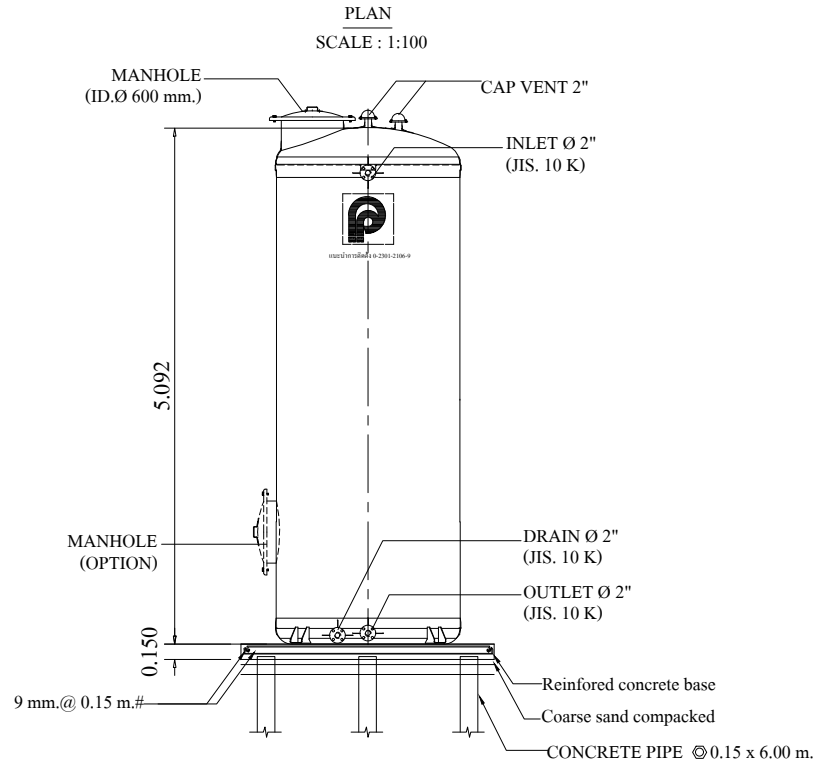
FRONT VIEW SCALE : 1:100
