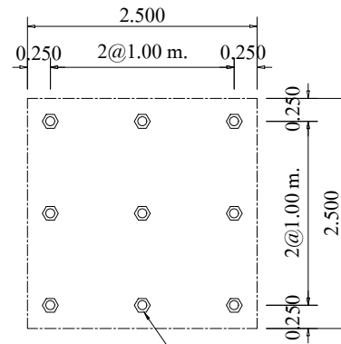
PLAN OF FOUNDATION SCALE : 1:100
