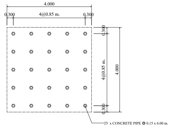
PLAN OF FOUNDATION SCALE : 1:100
