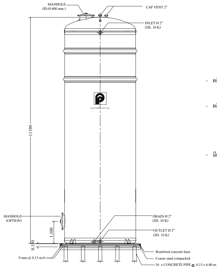
FRONT VIEW SCALE : 1:100
