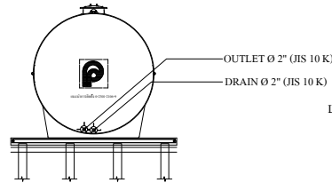
RIGHT VIEW
