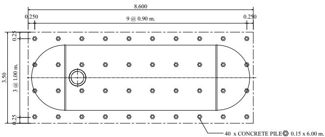
PLAN OF FOUNDATION SCALE : 1:100
