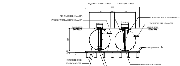
SECTION C-C SCALE 1 : 100
