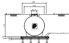
SIDE VIEW SCALE 1 : 100
