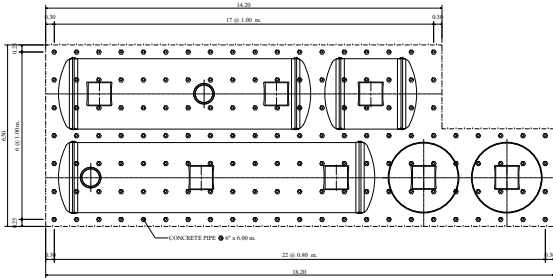
PLAN SCALE 1 : 100 SHOW LAY-OUT OF PILING
