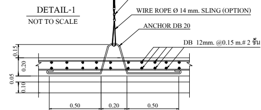
FIG.1 TANK TIGHTENING DETAIL. NOT TO SCALE
