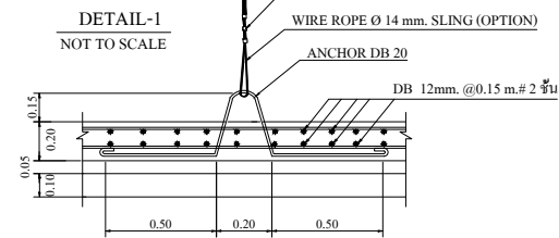
FIG.1 TANK TIGHTENING DETAIL. NOT TO SCALE
