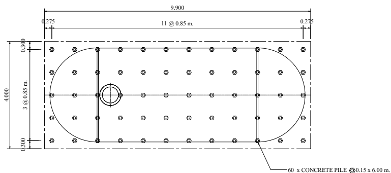
PLAN OF FOUNDATION SCALE : 1:100
