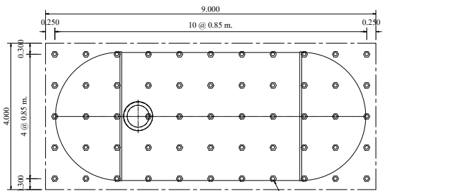
PLAN OF FOUNDATION SCALE : 1:100
