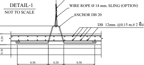
FIG.1 TANK TIGHTENING DETAIL. NOT TO SCALE
