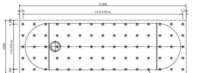
PLAN OF FOUNDATION SCALE : 1:100
