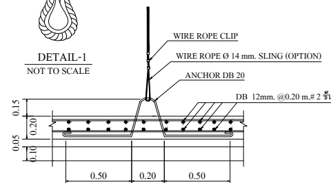
FIG.1 TANK TIGHTENING DETAIL, NOT TO SCALE
