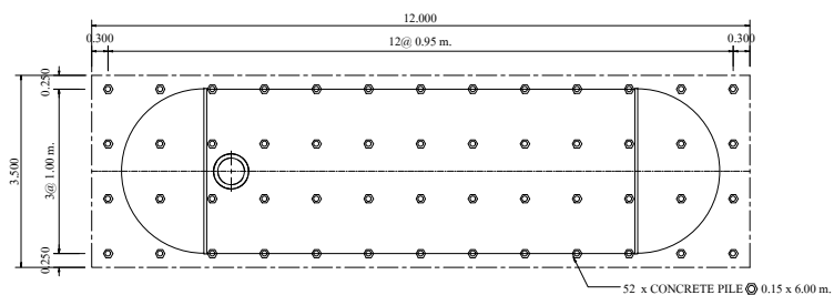
PLAN OF FOUNDATION SCALE : 1:100
