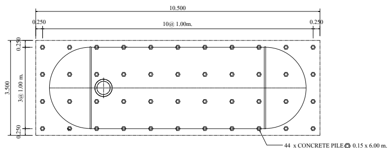
PLAN OF FOUNDATION SCALE : 1:100
