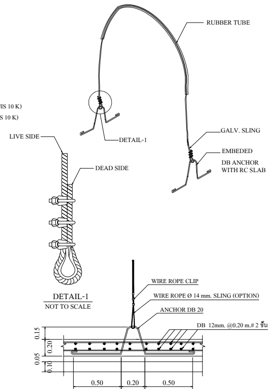
FIG.1 TANK TIGHTENING DETAIL, NOT TO SCALE
