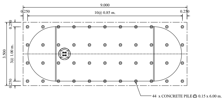
PLAN OF FOUNDATION SCALE : 1:100
