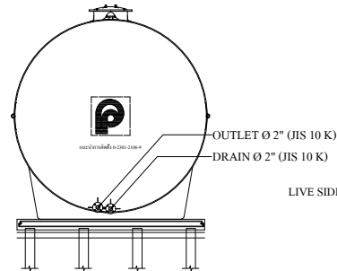
RIGHT VIEW
