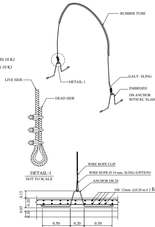
FIG.1 TANK TIGHTENING DETAIL. NOT TO SCALE
