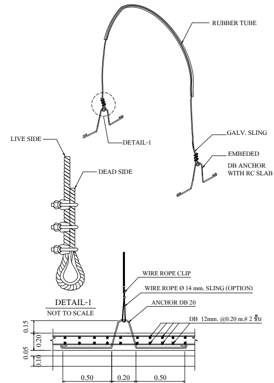
FIG.1 TANK TIGHTENING DETAIL. NOT TO SCALE
