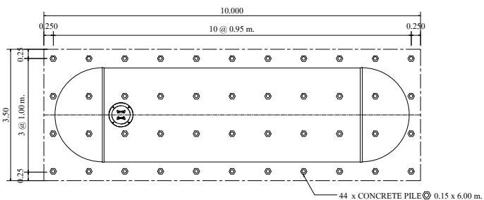
PLAN OF FOUNDATION SCALE : 1:100
