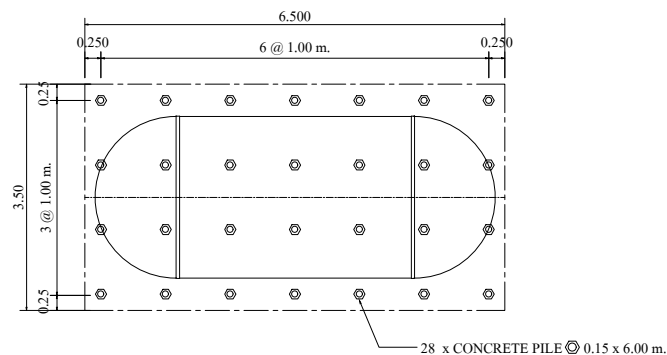
PLAN OF FOUNDATION SCALE : 1:100
