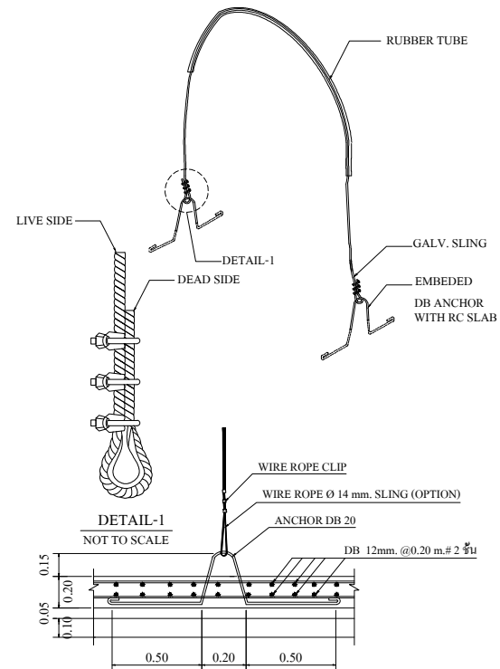
FIG.1 TANK TIGHTENING DETAIL. NOT TO SCALE
