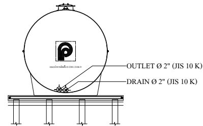
RIGHT VIEW
