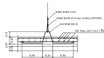
FIG.1 TANK TIGHTENING DETAIL NOT TO SCALE
