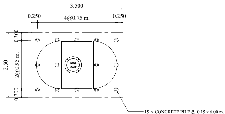
PLAN OF FOUNDATION
