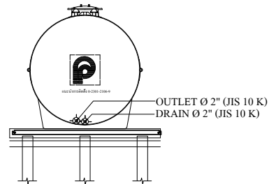
RIGHT VIEW
