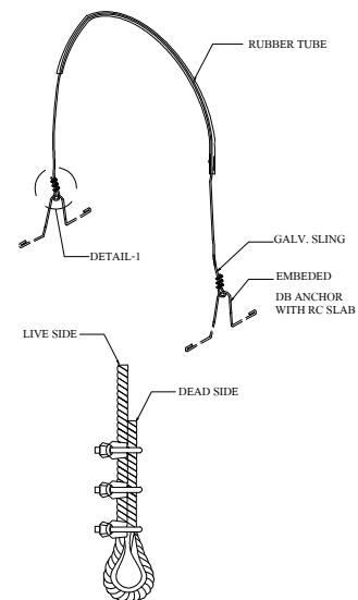
DETAIL-1 NOT TO SCALE
