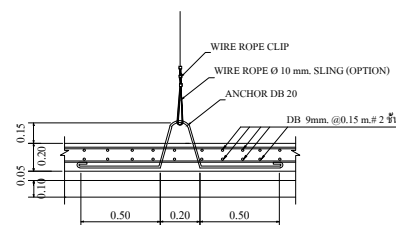
FIG.1 TANK TIGHTENING DETAIL. NOT TO SCALE
