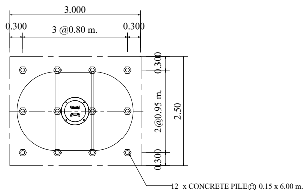
PLAN OF FOUNDATION
