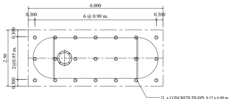
PLAN OF FOUNDATION
