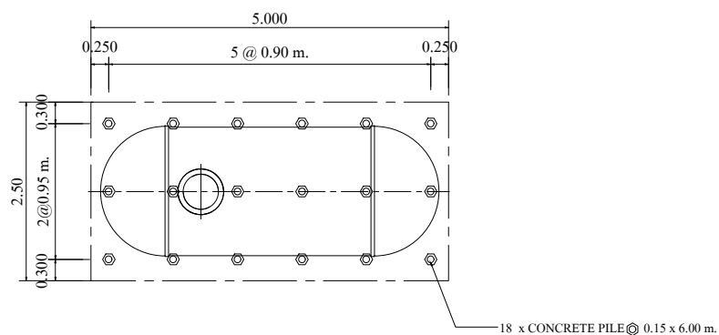
PLAN OF FOUNDATION
