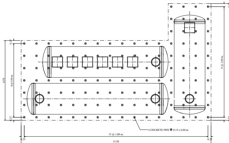
PLAN SCALE 1:100 SHOW LAY-OUT OF PILING
