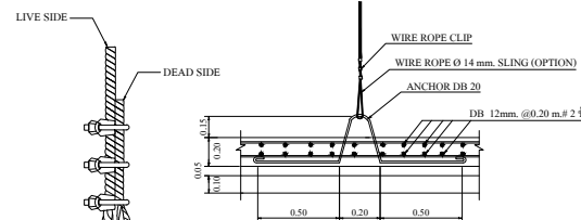
FIG.1 TANK TIGHTENING DETAIL. NOT TO SCALE
