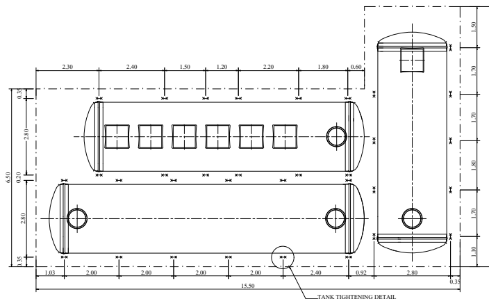
PLAN SCALE 1:100 SHOW LAY-OUT OF PILING
