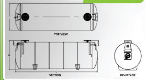
EC-60E(S) to 75E(S)
